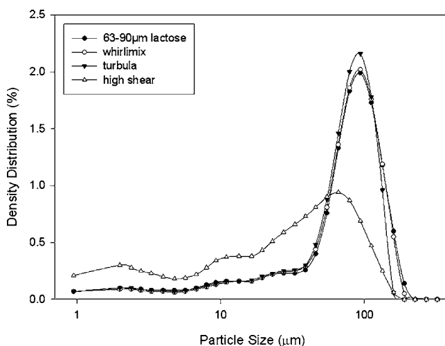
Fig. 2. Particle size distribution of the sieved 63–90 \mu\text{m} \alpha -lactose monohydrate before and after, whirlmixer, turbula and high shear processing.
